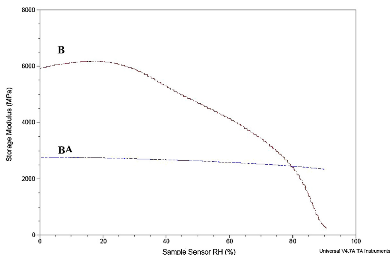
Fig. 7. Mechanical properties of bleached (B) and bleached-acetylated film (BA) against humidity.
