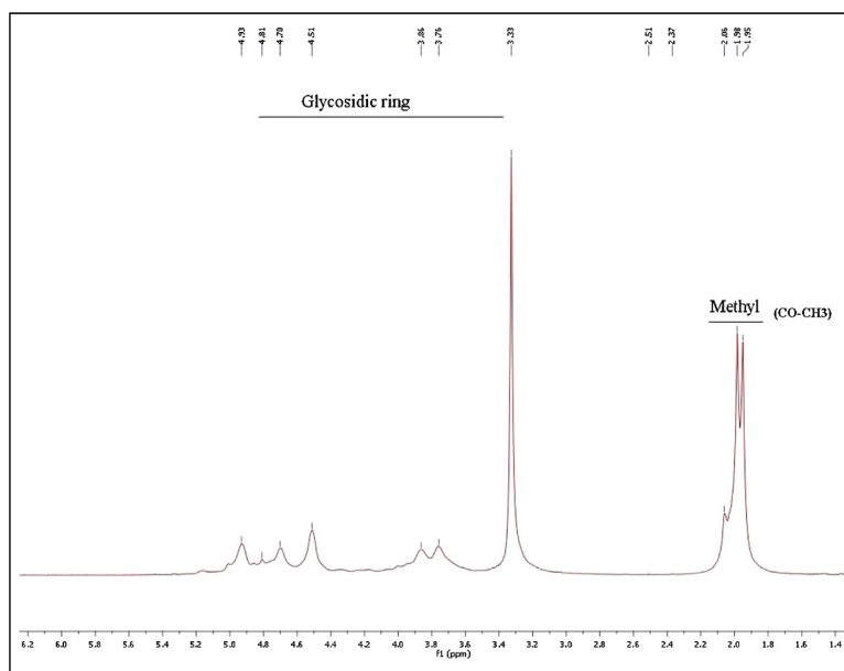
Fig. 6. ^1\text{H} NMR spectrum of bleached-acetylated CCAX (dissolved in \text{DMSO-d}_6 ).
