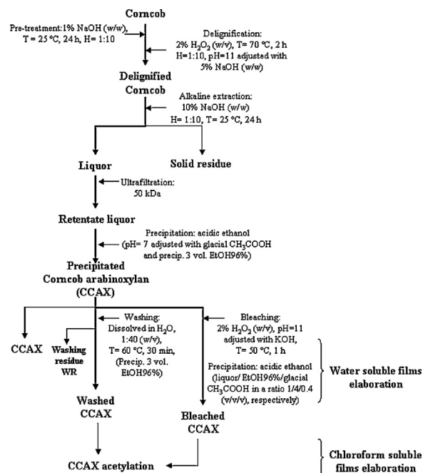
Fig. 1. Scheme of corn cob arabinoxylan extraction, purification treatments, acetylation and film elaboration.
